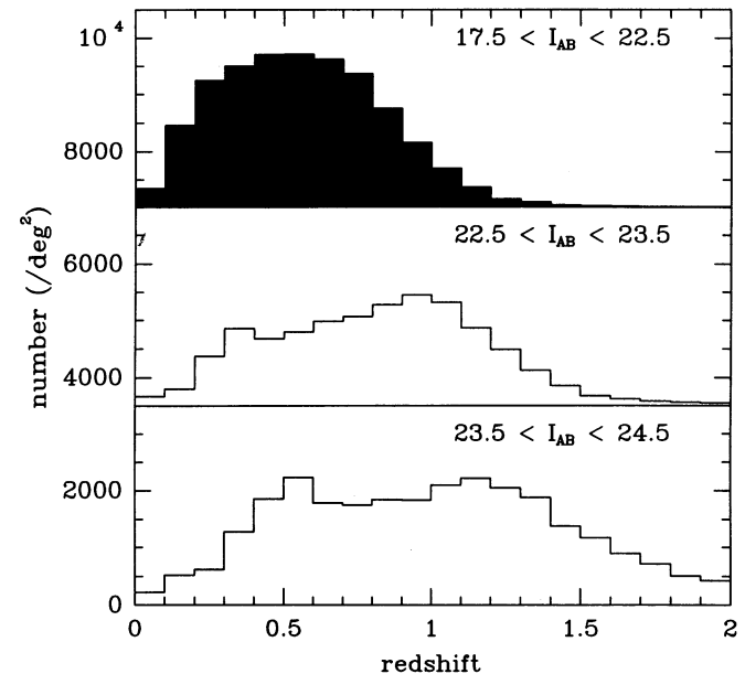
FIG. 9.—The N(z) distributions obtained from the CFRS luminosity function in the 17.5 < I_{AB} < 22.5 range (upper histogram) and extrapolated, assuming no further evolution, to fainter magnitudes, 22.5 < I_{AB} < 23.5 and 23.5 < I_{AB} < 24.5 .
